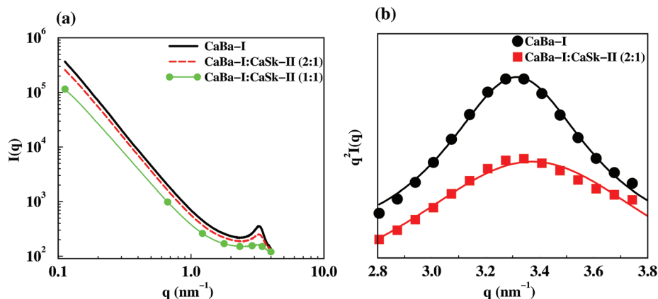
Fig. 7 (a) Scattering intensity as a function of wave vector for CaBa-I (solid line), and for CaBa-I and CaSk-II mixed in mass ratios of 2 : 1 (long dashed line) and 1 : 1 (green solid line with symbols). (b) The fitting procedure gives tactoid sizes of \approx 10 and \approx 6 . The dispersion with mass ratio 1 : 1 has a too broad peak to be analyzed. The solid lines are obtained from eqn (1).
