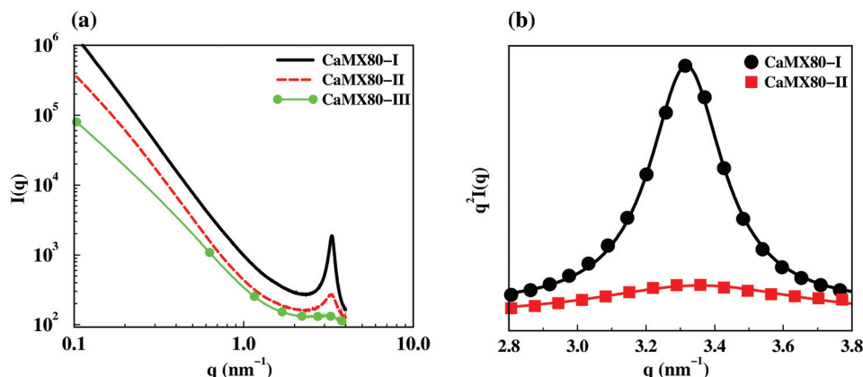
Fig. 4 (a) Scattering intensity as a function of wavevector for different CaMX80 fractions obtained from NaMX80 through equilibration with a 0.5 M \text{CaCl}_2 solution. MX80-I is shown as black solid line, MX80-II red dashed line and MX80-III green solid line with symbols. (b) Fitting of the SAXS peak for MX80-I gives N \approx 25 (solid black line) and for MX80-II N \approx 9 (red dashed line). The peak for MX80-III is too broad to be analyzed. The solid lines are fits obtained from eqn (1) and symbols are measured values.
