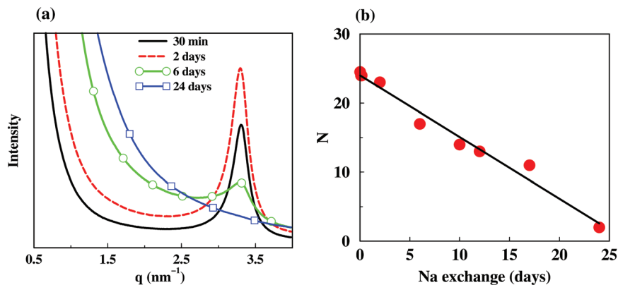
Fig. 5 (a) SAXS spectra from CaMX80-I dispersion equilibrated with a 50 mM NaCl solution for increasing time intervals from 30 min to 24 days as indicated in the graphs. (b) The number of platelets per tactoid, N , as a function of time for the system in (a).
