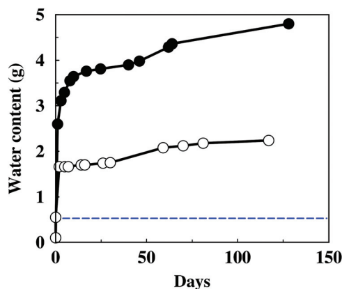
Fig. 3 Swelling of fractionated and unfractionated Ca montmorillonites. Dry powder (1 g) of CaMX80 obtained by ion exchange from fraction I of NaMX80 (open circles) and from unfractionated CaMX80 (filled circles) were placed in dialysis pockets and immersed in millipore water. The blue dashed line indicates the intra-lamellar swelling.
