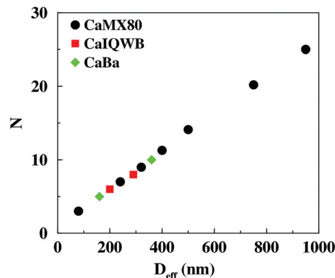
Fig. 9 Tactoid size, N , as a function of effective platelet size, D_{\text{eff}} for size fractionated clays of different natural origin.
