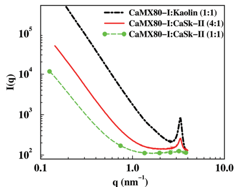
Fig. 8 (a) Scattering intensity I(q) as a function of wave vector for a mixture of CaMX80-I and kaolin, and for a mixture of CaMX80-I and CaSk-II with mass ratios (4 : 1) and (1 : 1) as indicated in graph.
